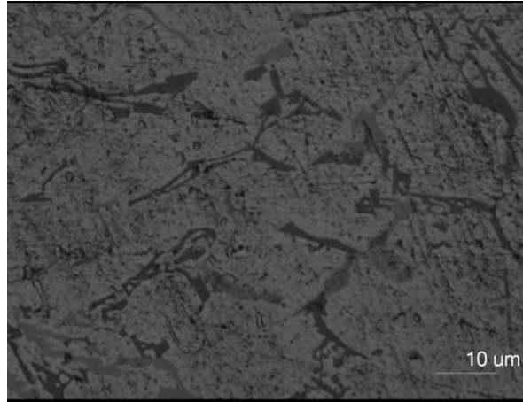
Figure 64: Aluminum Sample Microstructure with Scale 10 µm and at 100X Magnification.
