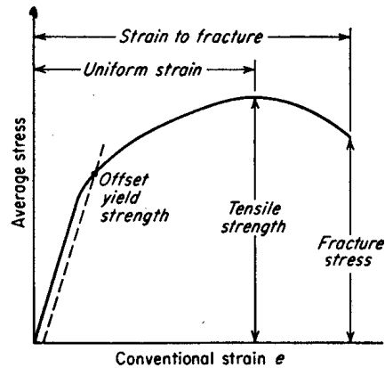
Figure 31: Stress-Strain Graph.
