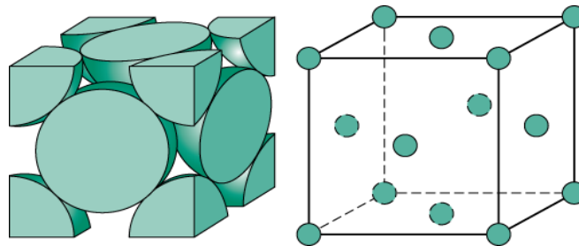
Figure 35: Face Centered Cubic Crystal Structure.
