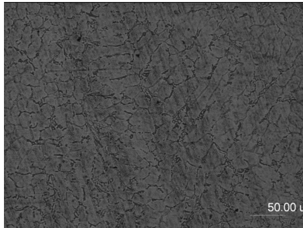
Figure 65: Aluminum Sample Microstructure with Scale 50 µm and at 20X Magnification
