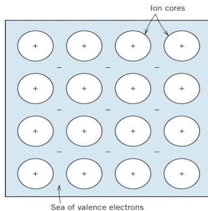
Figure 33: Metallic Bonding.
