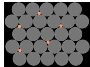
Figure 37: Interstitial Atoms
