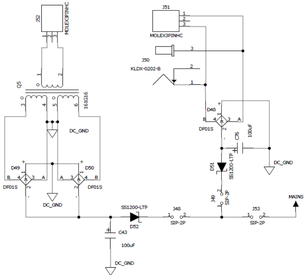
Figure 61 – AC Power Circuit
