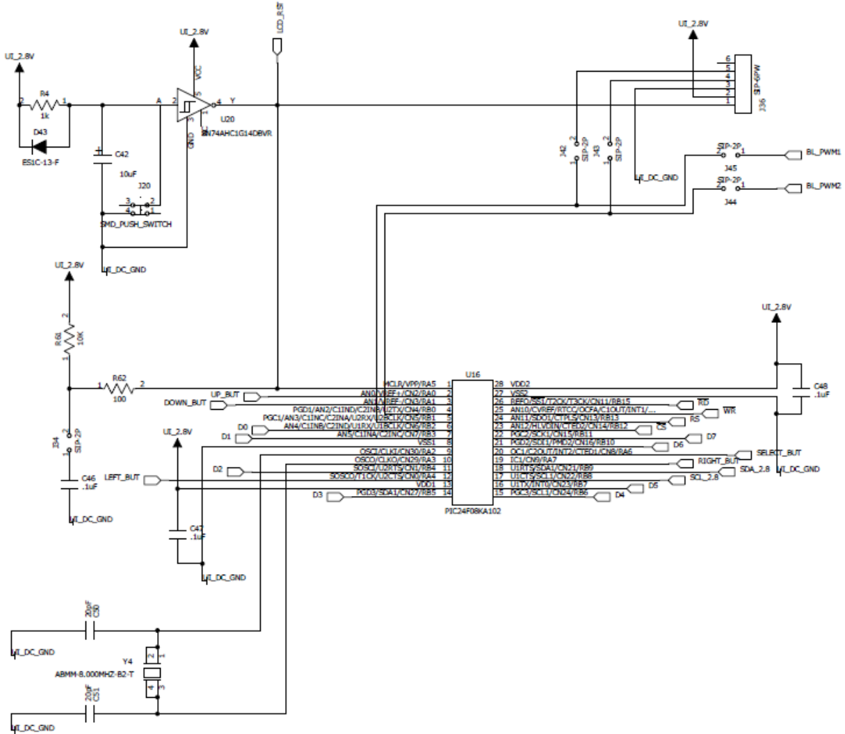
Figure 64 – Interface Controller Circuit
