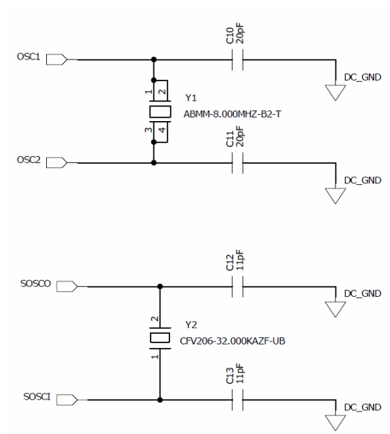
Figure 37 – Oscillator Circuits
