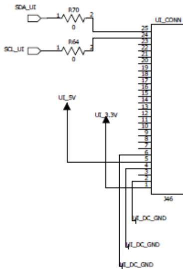
Figure 62 – Master Connector Circuit: UI Side
