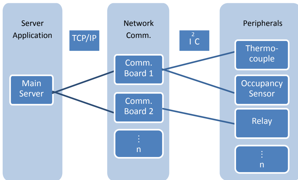
Figure 9: New System Architecture
