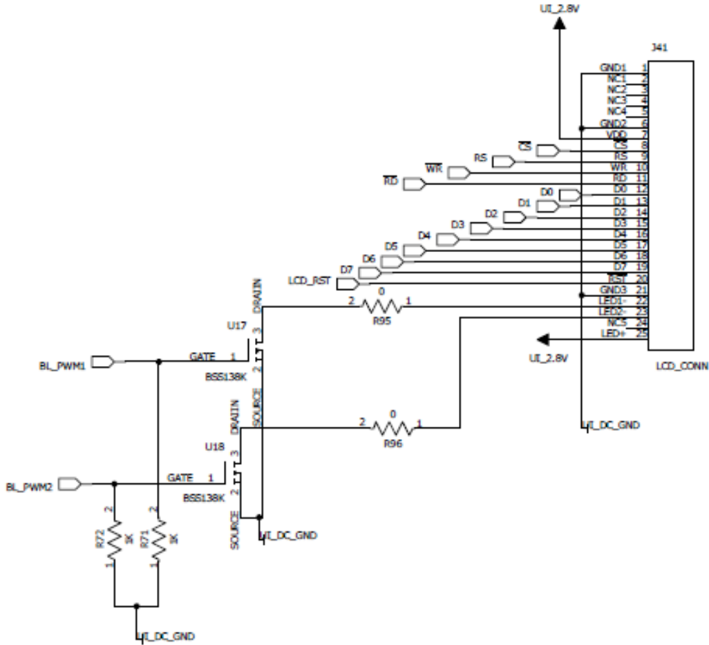
Figure 65 – Liquid Crystal Display (LCD) Circuit
